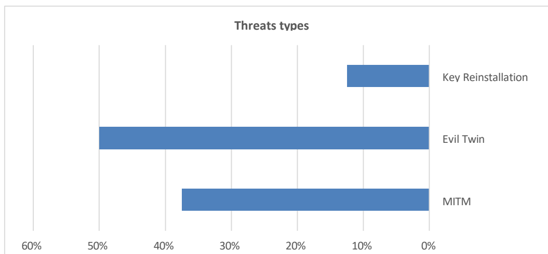
Figure 5. Findings of the most common types of Cyber threats and attacks on Confidentiality
