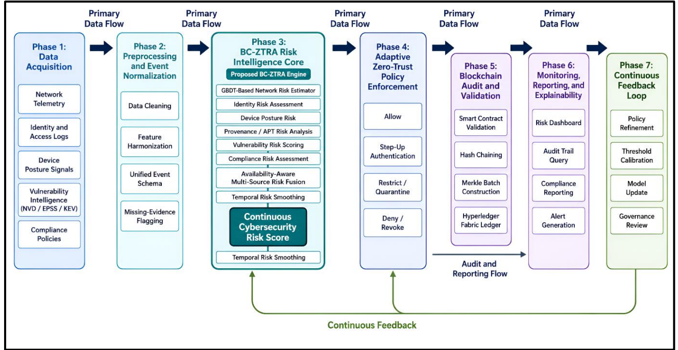
Figure 2. Phase-wise workflow of the proposed BC-ZTRA algorithm.
