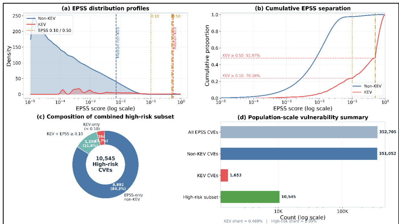
Figure 8. EPSS distributions of KEV and non-KEV vulnerabilities and composition of the combined high-risk vulnerability subset.
