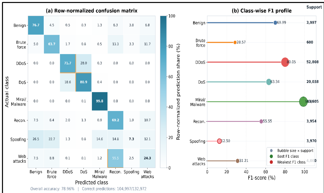
Figure 5. Normalized confusion matrix and class-wise F1 profile of the GBDT network-risk estimator used within BAZTRA.
