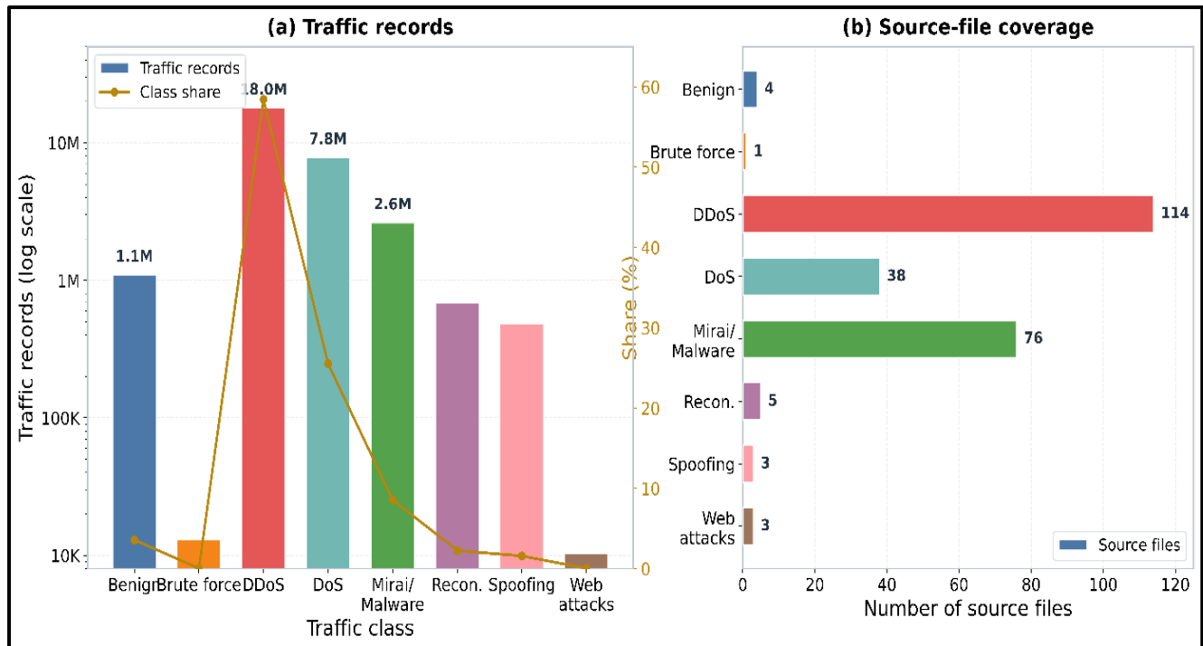
Figure 3. Log-scaled distribution of traffic records and source-file coverage across the eight CICIOT2023 classes.
