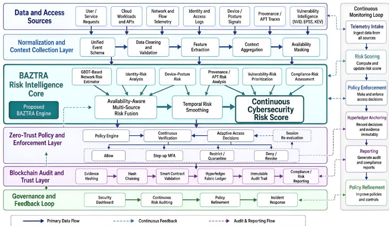
Figure 1. Layered architecture of the proposed blockchain-enabled zero-trust cloud-security and continuous cybersecurity-risk auditing framework.
