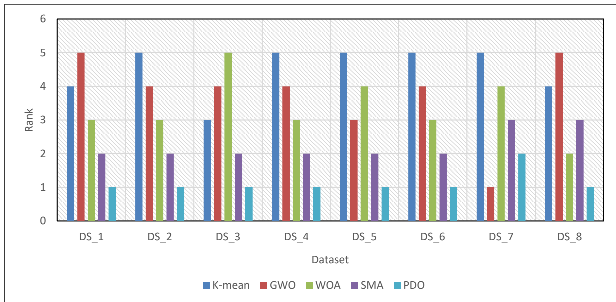
Figure 2 Average rankings of the algorithms used to select text features.
